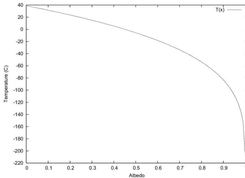
Figure 10 Earth's average surface temperature at different values of the albedo
